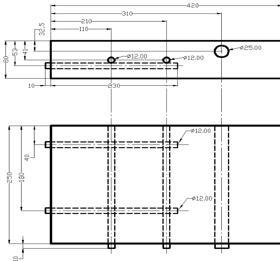
Detection block
